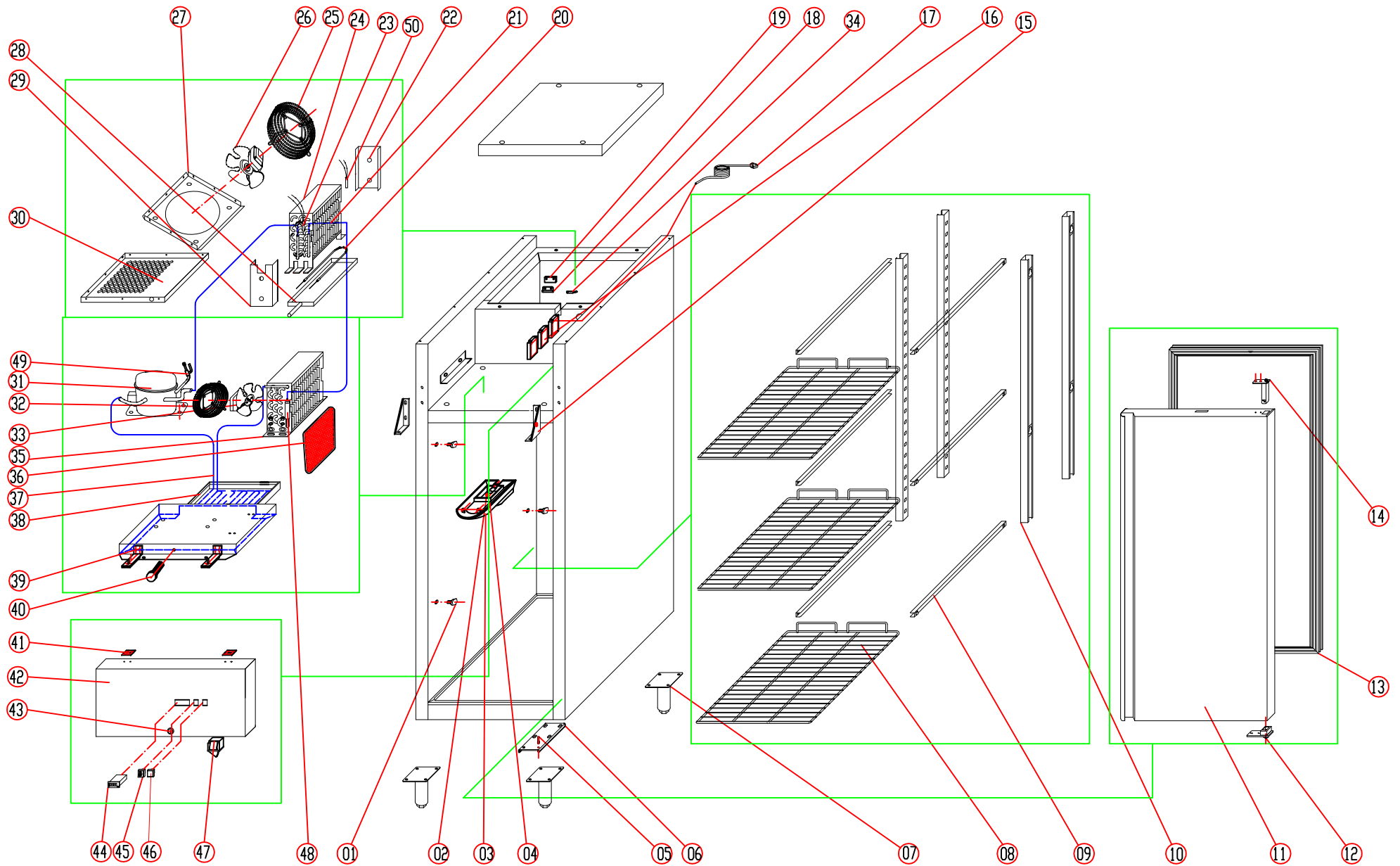
EXPLODED VIEW OF GN650BT
